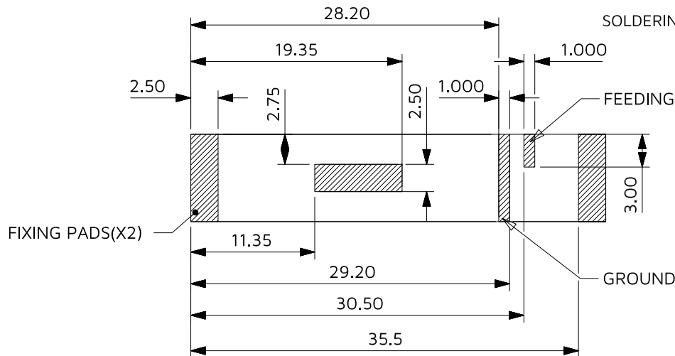
PADS OF PRODUCT FOR SOLDER
